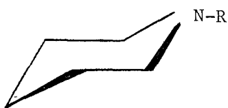
Figure 4-1 Substituted piperidine ring found in all opiates (natural and synthetic)
