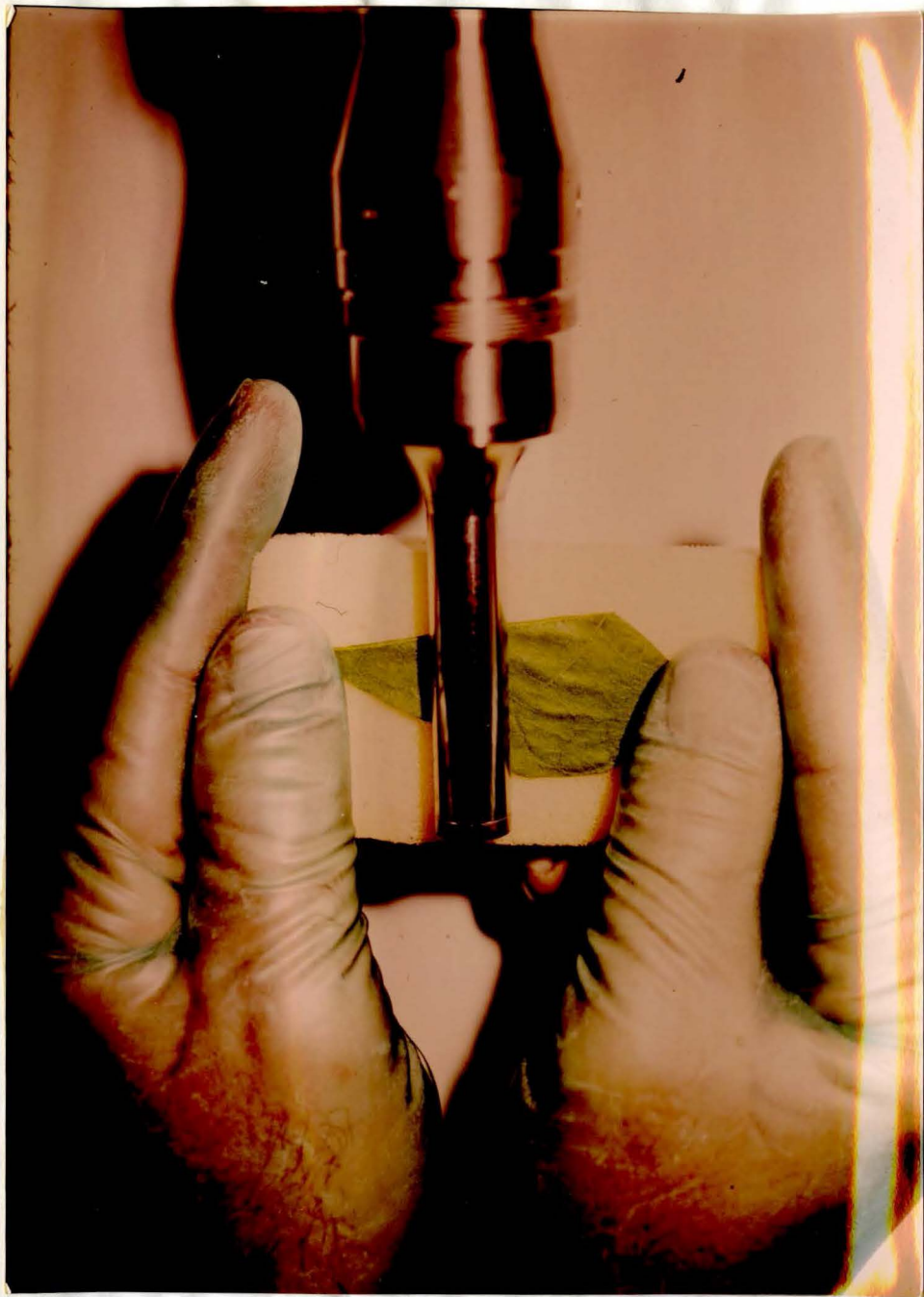
Figure 8. Ultrasonic inoculation of a half leaf of Phaseolus vulgaris cv pinto, with extract treated TMV. Leaves were pass through under the sonic probe with even pressure.
