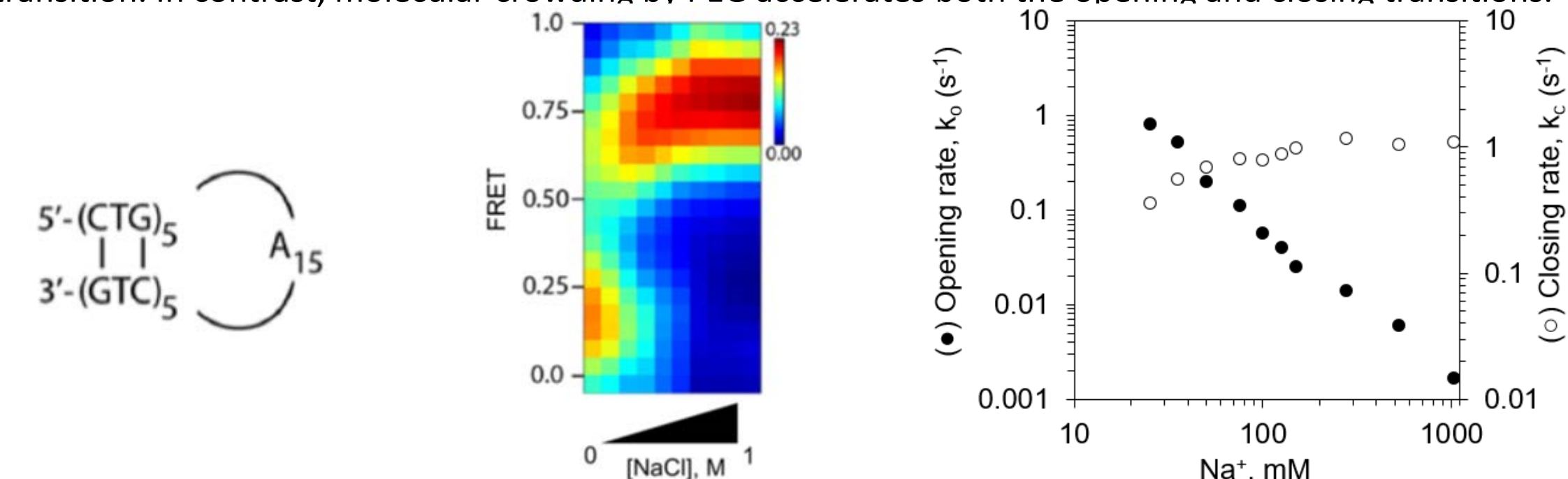
Figure 3. Increasing NaCl levels promotes stabilization of the closed hairpin conformation (CTG) 5 . Analysis of the transition kinetics reveals this occurs primarily through slowing of the opening transition.
