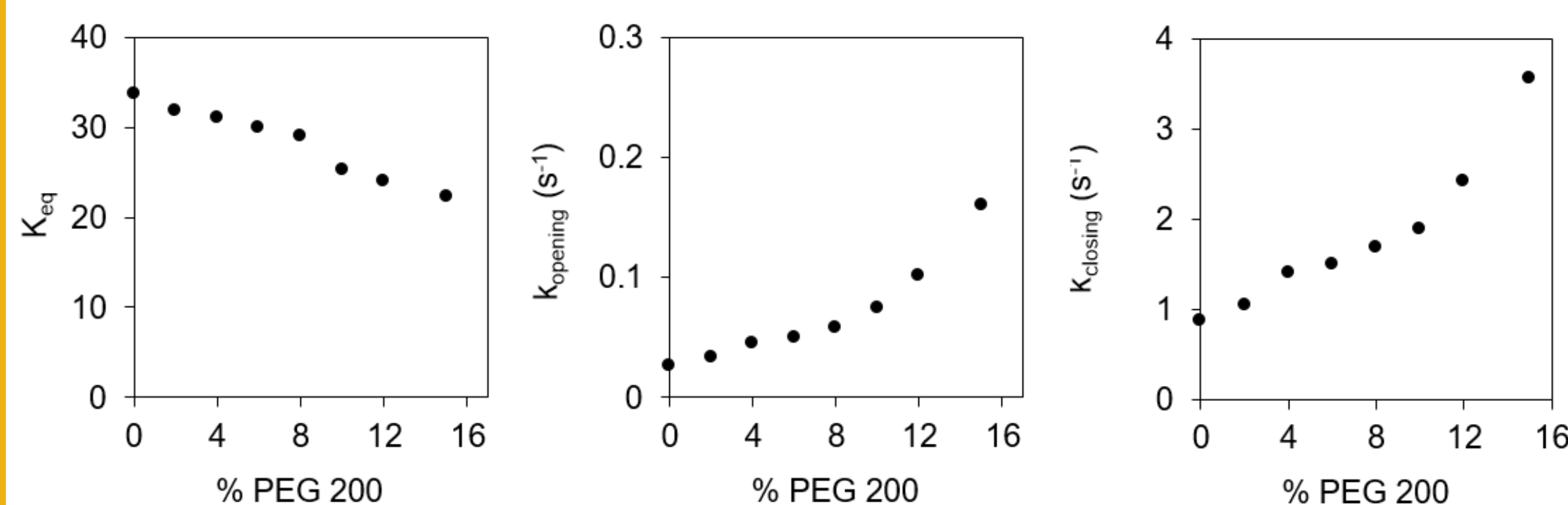
Figure 5. Contrasting effect of PEG on hairpin in higher salt. The measured equilibrium constants ( K_{eq} ) and transitions rates for (CTG) 5 hairpins in increasing concentrations of PEG 200 in 100 mM NaCl.
