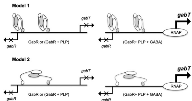
Fig. 7. A model for transcriptional regulation at the gabR and gabT promoters. Different models for GabR binding in the gabR-gabT regulatory region are depicted. The GabR homodimer is represented as a cartoon with one monomer shown in white and the other colored gray. The larger oval represents the AT-fold domain and the smaller oval represents the winged-helix domain. Putative conformational changes in the presence of GABA are indicated by symbols with dashed lines.
