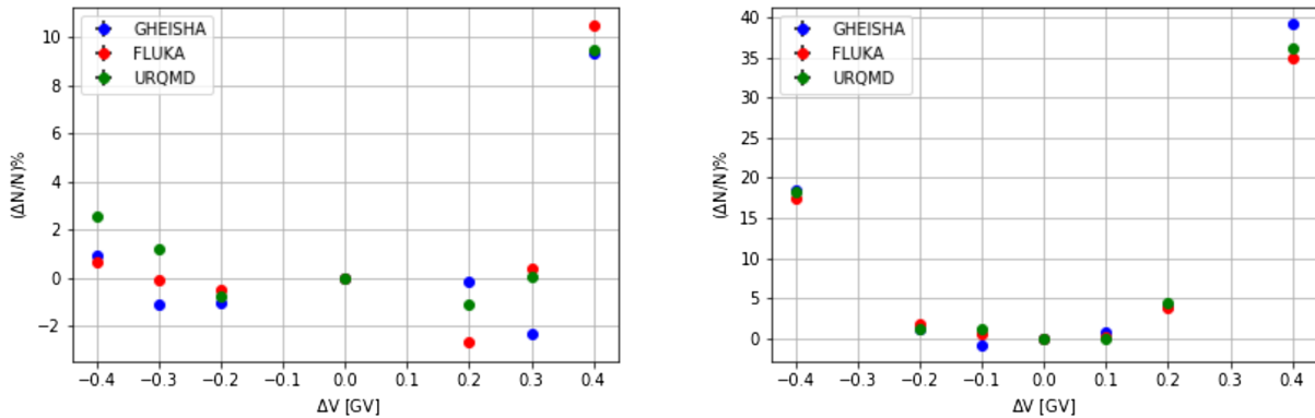
FIG. 5. Left: (\Delta N/N)\% vs \Delta V , including statistical error, for a uniform electric field layer inside the cloud ( IntraCloud model ) using the three low energy model GHEISHA, FLUKA, and URQMD. The model uses a uniform electric field 2 km inside the thundercloud that is located 2 km above ground level. Right: (\Delta N/N)\% vs \Delta V , including statistical error, for a uniform electric field layer between the cloud and ground ( Cloud-to-Ground model ) using the three low-energy model GHEISHA, FLUKA, and URQMD. In this model the thundercloud base is 2 km in height from the detector.
