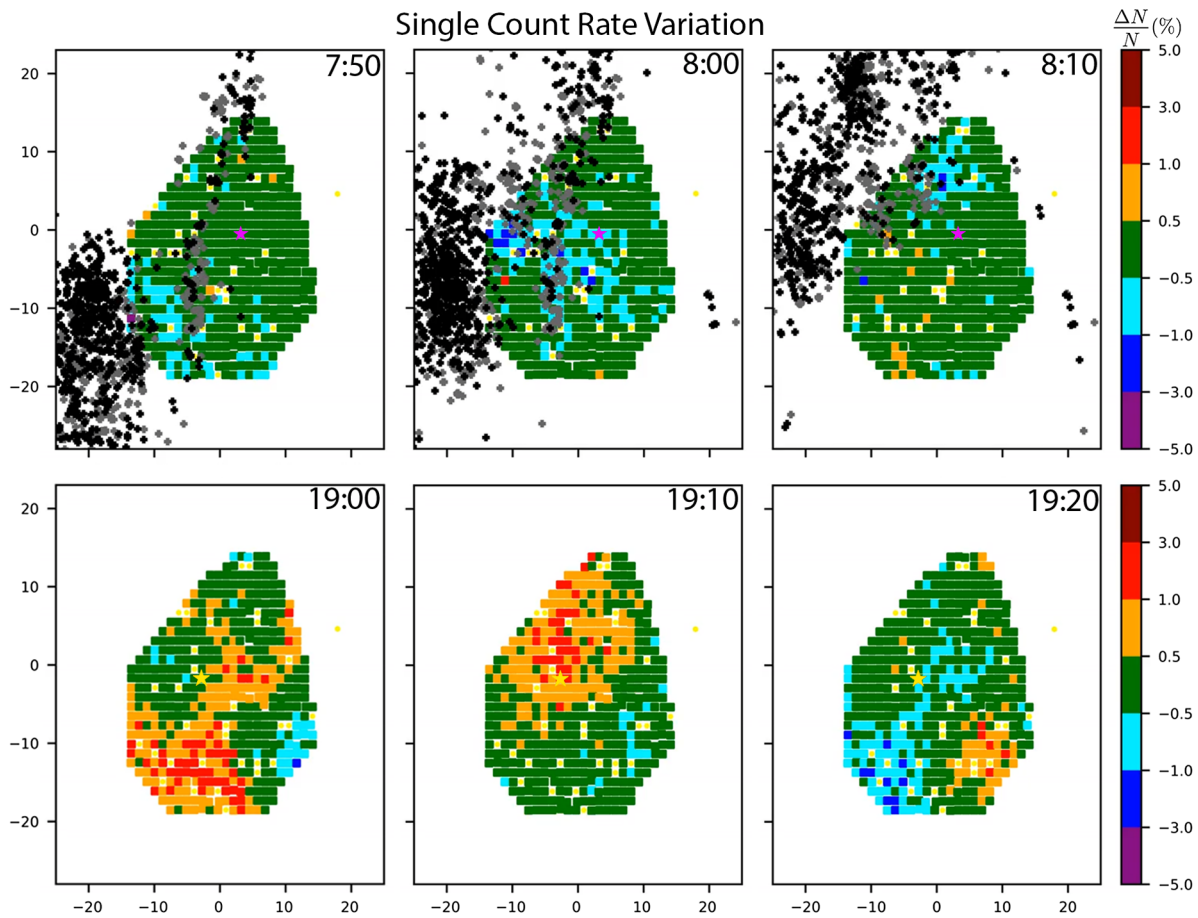
FIG. 2. Time evolution of the intensity variation of the single count rate change ( \frac{N_c - N_p}{N_p} )% or ( \Delta N/N )% on the 09/27/2014 thunderstorm. Each time frame is ten minutes in duration. The starting time in UTC is denoted on each frame. The black and gray crosses marks are the intracloud and cloud-to-ground lightning sources detected by the NLDN for each frame. The two yellow and pink stars point at the two detectors [1516 (denoted in pink) and 1015 (denoted in yellow)] plotted in Fig. 3.
