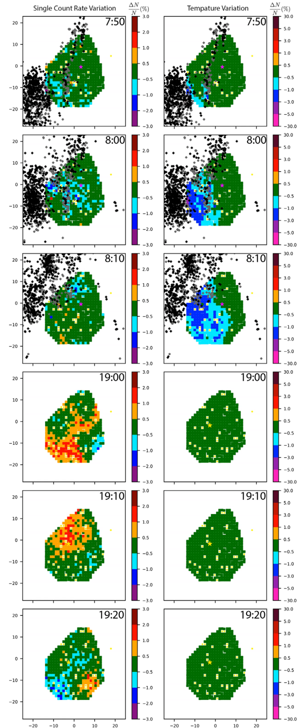
FIG. 7. Left: Time evolution of the intensity variation of the secondary low-energy cosmic-ray counting rate change ( \frac{N_c - N_p}{N_p} ) or ( \Delta N/N ) on the 09/27/2014 thunderstorm shown in Fig. 2. Right: Temperature variation at 1400 m ( T_c - T_p ) or ( \Delta T ) for the same frames. T_c is the temperature in the current frame and T_p is the temperature in the previous frame. The starting time is denoted on each frame. The black and gray cross marks are the intracloud and cloud-to-ground lightning sources detected by the NLDN for each frame.
