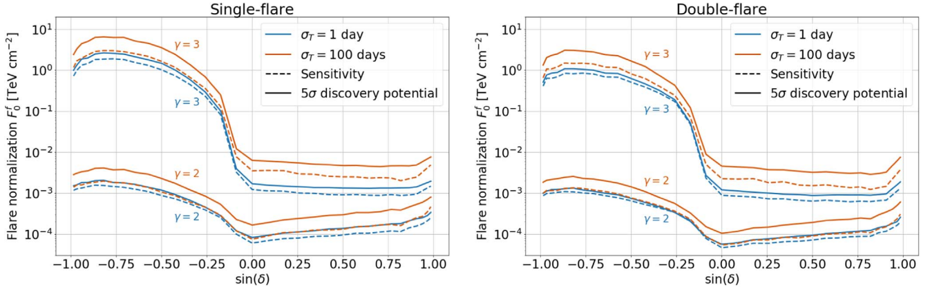
Figure 5. Sensitivity (dashed lines) and 5\sigma DP (solid lines) of the multi-flare analysis vs. decl., expressed in terms of the flux normalization factor per flare F_0^f defined in Equation (A1), under the hypothesis of a single (left plot) and a double (right plot) signal flare. The assumed energy dependence of the flares has a spectral index of \gamma^f = 2 and \gamma^f = 3 (see labels), and a flare duration of \sigma_T^f = 1 day (blue lines) and \sigma_T^f = 100 days (orange lines). The double-flare assumes two identical and well-separated flares.
