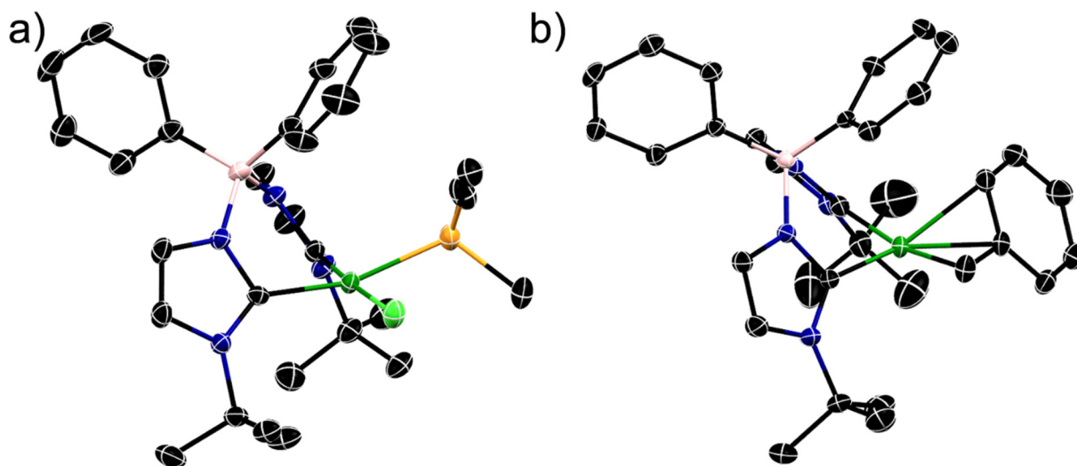
Figure 3. X-ray crystal structures of (a) \text{Ph}_2\text{B}(\text{}^t\text{BuIm})_2\text{NiCl}(\text{PMe}_3) , selected bond lengths ( \text{\AA} ): Ni-Cl 2.2205(9); Ni-P 2.219(1); Ni-C 1.921(3); 1.862(3); and (b) \text{Ph}_2\text{B}(\text{}^t\text{BuIm})_2\text{Ni}(\eta^3\text{-C}_7\text{H}_7) , selected bond lengths ( \text{\AA} ) and angles ( ^\circ ): Ni-C (carbene) 1.916(2); 1.876(2). Ni-C (benzyl) 1.974(2), 2.100(2), 2.228(2) Thermal ellipsoids shown at 50 % probability, hydrogen atoms omitted for clarity. Black, blue, red, light green, pink, green and orange ellipsoids correspond to C, H, O, Cl, B, Ni and P atoms, respectively.
