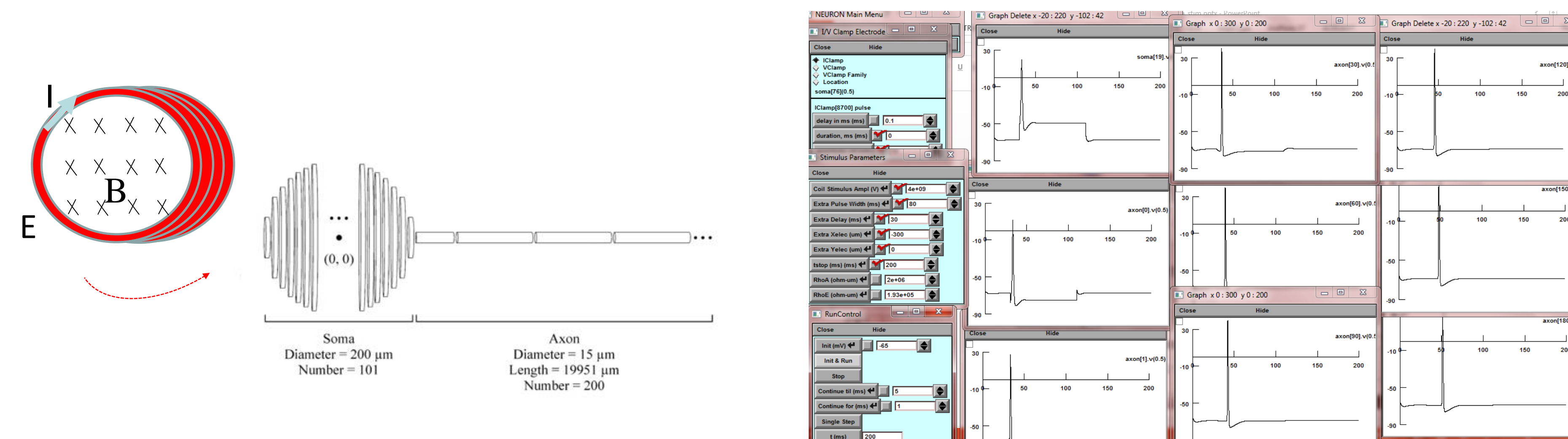
Figure 8. NEURON simulation with the coil over the soma producing a 4e+09 V pulse can produce action potentials in the soma. The action potentials propagate down the axon over time.
