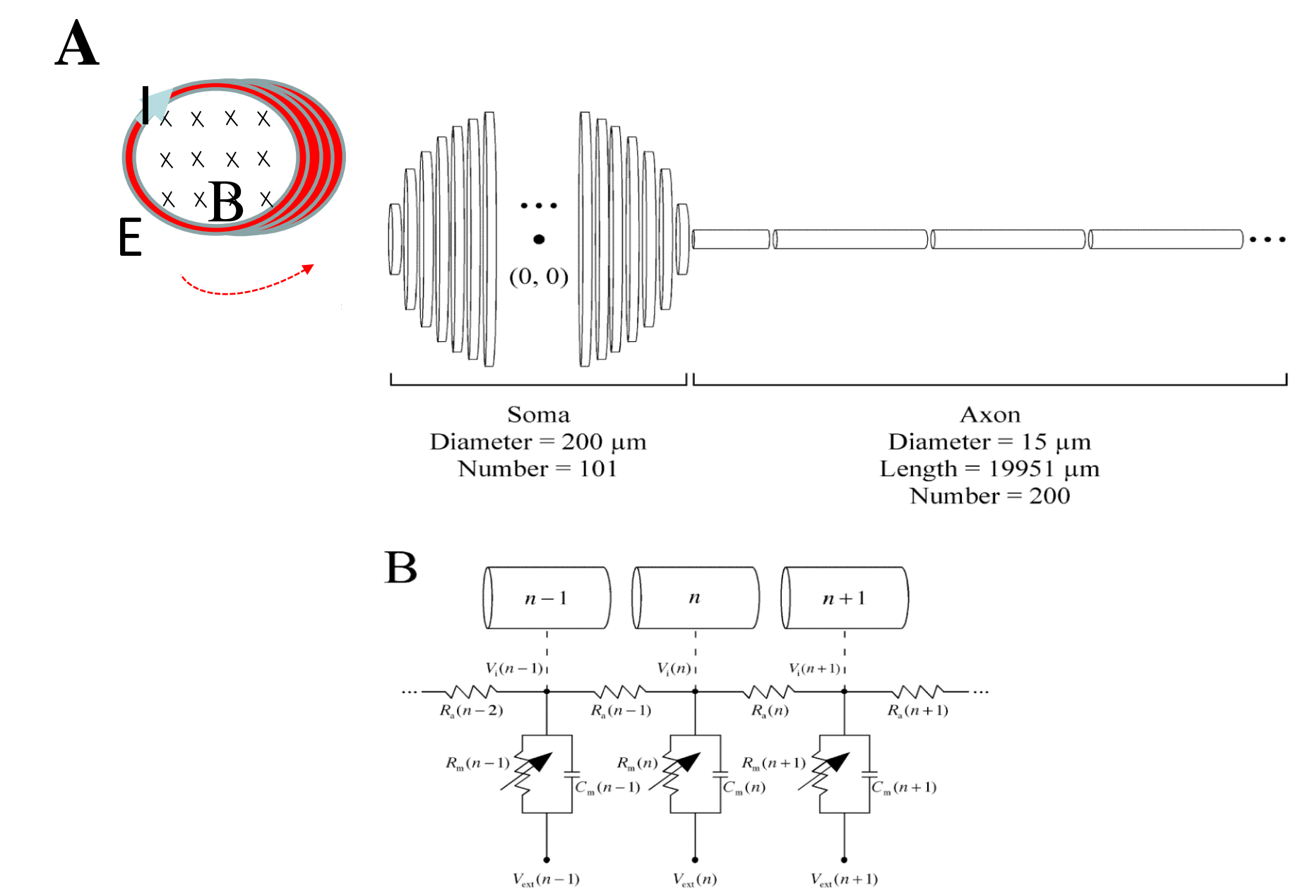
Figure 6. A. Multicompartment model for magnetic stimulation modified from Lu 2008. The soma is composed of 101 segments whose center is at (0,0). The axon is composed of 200 segments and reaches 19951 μm. The coil is positioned over the soma (not to scale). B. The passive neuron properties used in the axon as described in Huxley 1952.
