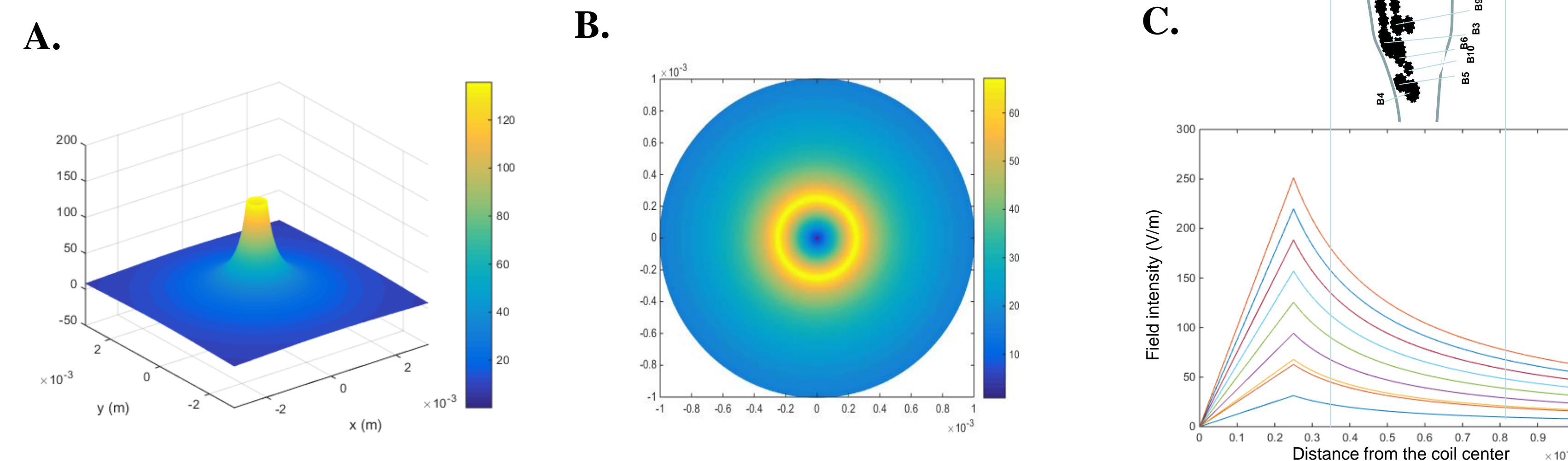
Figure 5. Computation of induced electric field around the mini coil. A. Intensity of the induced electric field inside and outside of the mini-coil in 3D space. Color map plot for the field intensity and its distribution around the coil, with the brightest, most intense induced field being inside the coil. B. Intensity of the induced electric field inside and outside the mini coil in 2D space. With the same color distribution as in [A]. C. The intensity of the electric field (in V/m) compared to distance from the coil center. The peak is inside the coil, while the ganglion will experience intensities between the 2 blue lines. Each color graphed represents a different stimulation intensity.
