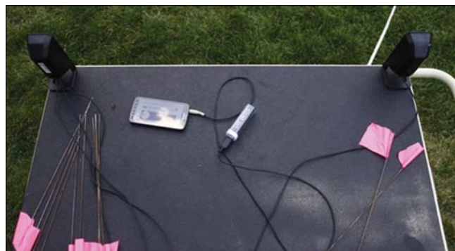
Fig. 1. The two speakers are placed on a cart about 1 m above the ground. The signal is provided by a smartphone, and the speakers are powered by a battery pack. Stake flags are also shown on the cart.
