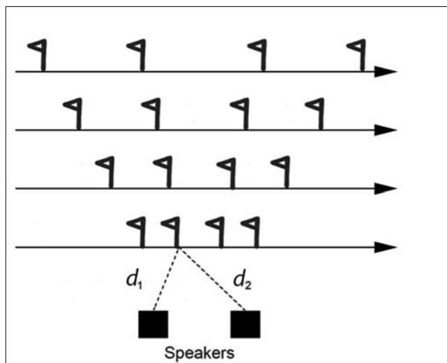
Fig. 2. Students follow the path shown by the arrowed lines, placing stake flags at points of destructive interference. Each arrowed line is parallel to a line connecting the two speakers. By following the paths shown and continually increasing the distance from the two speakers, a clear interference pattern, shown by the flags, is formed. The wavelength of the sound wave is determined by measuring the distance from each speaker, denoted by d_1 and d_2 , to a nearby flag.
